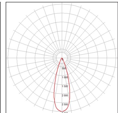
Curva 1 LED 2W- facho 40°
